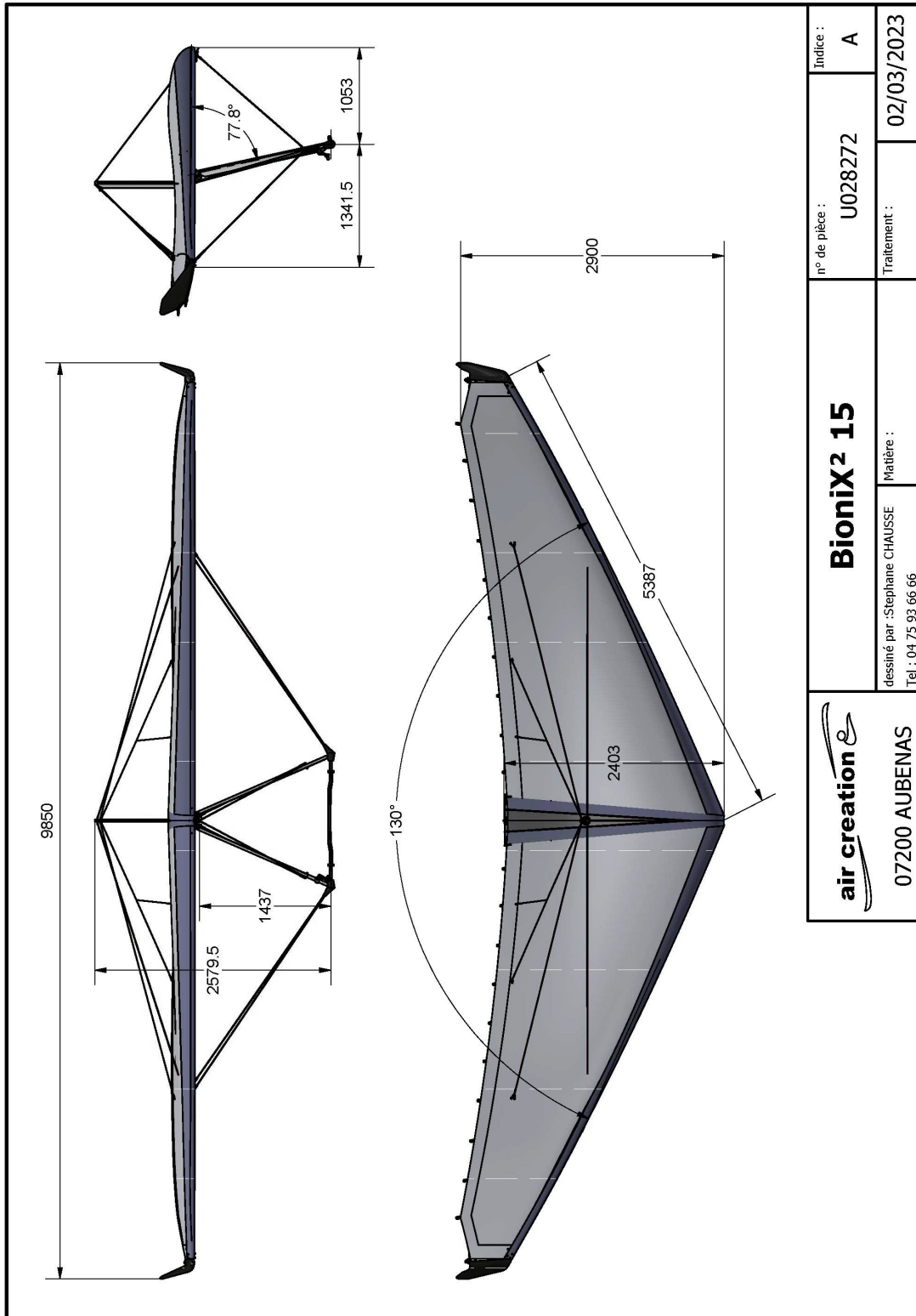
Figure 3-1: BioniX 2 15 in 3 Perspectives
